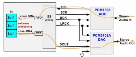
Fig. 7 datapath audio
